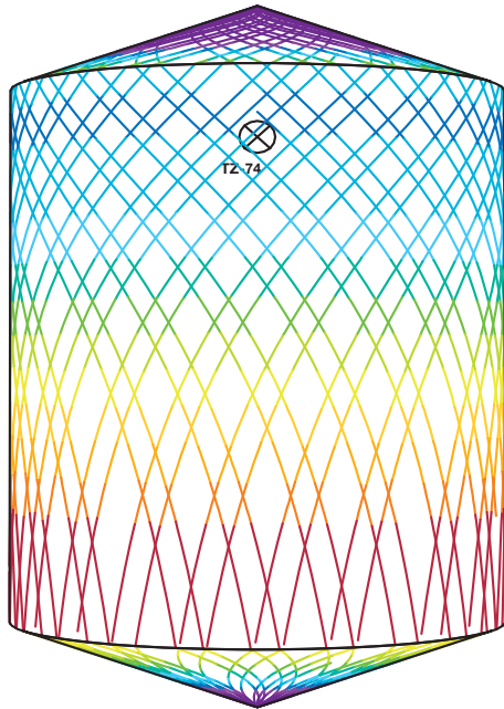
D5m H6m, Toftejorg TZ-74 Self Cleaning version, 4 x ø7 mm, 0% Time = 3.8 min., Water consumption = 1192 l
